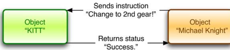
Figure 3.5. Passing arguments
