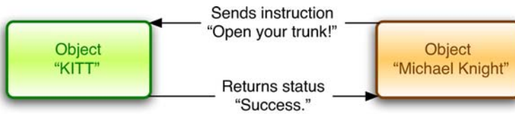
Figure 3.4. Sending instructions
