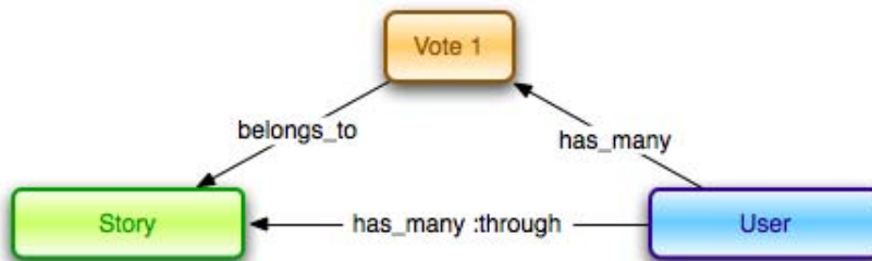
Figure 9.9. A join model relationship
